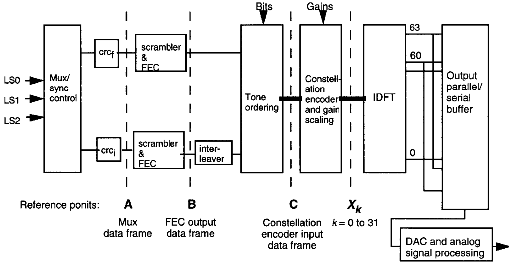
Figure 3 – ATU-R transmitter reference diagram
