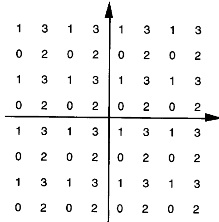
Figure 13 – Constituent 2-dimensional cosets for Wei's code
