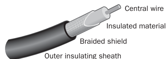
Coaxial cable.
