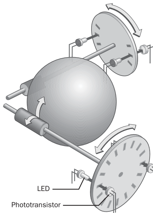
Optomechanical mouse.
