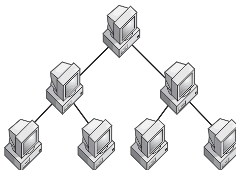
Tree network.
