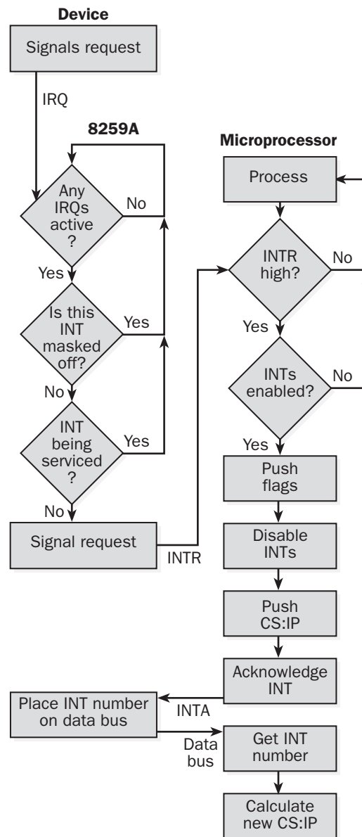
Flowchart.
