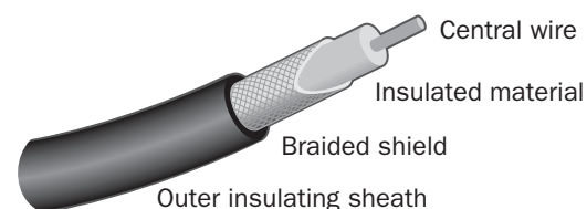
Coaxial cable.
