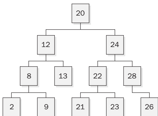
Binary tree.
