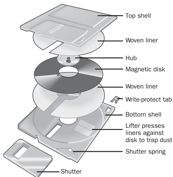
Exploded view.
