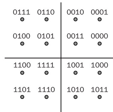
Constellation.
