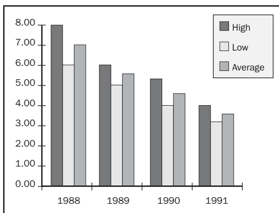
Column chart.
