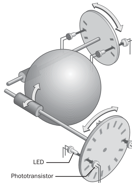
Optomechanical mouse.
