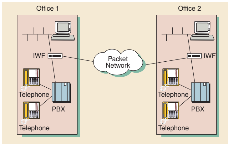
Fig. 3 Application 2: interoffice trunking
