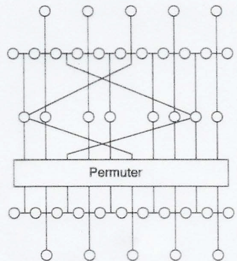
Irregular turbocode R=8/18
