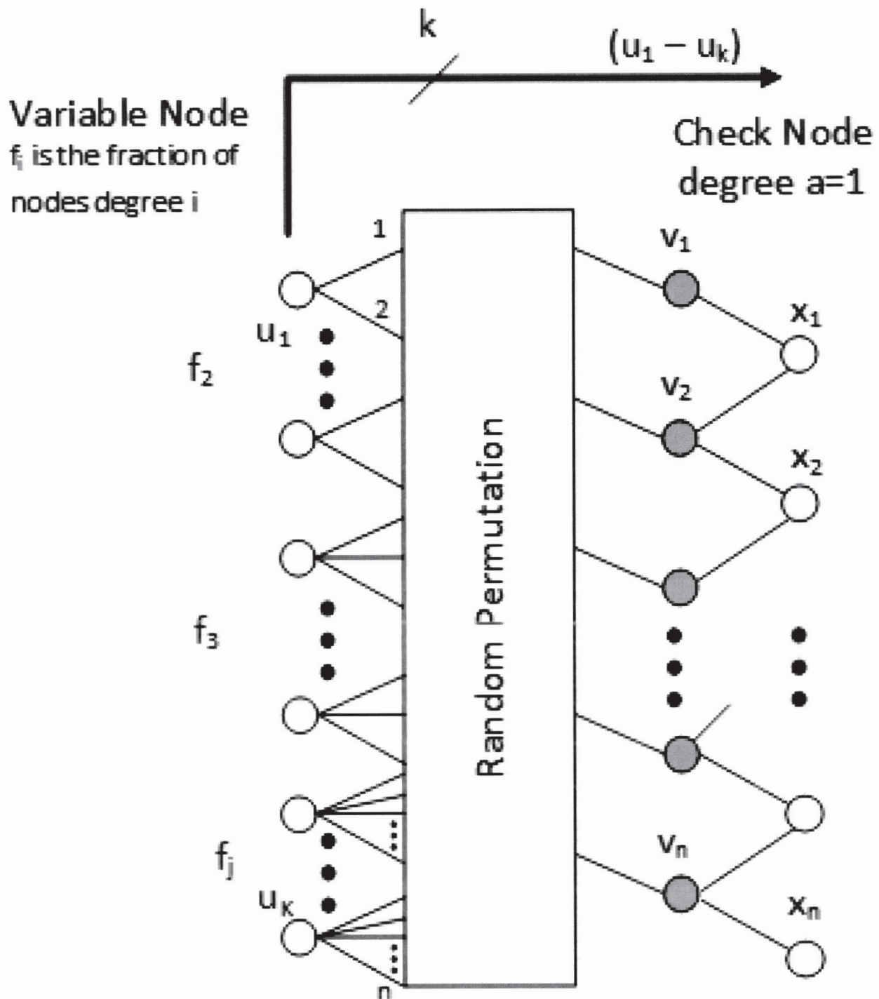
Tanner graph for a code described by Fig. 2 of '710 Patent
