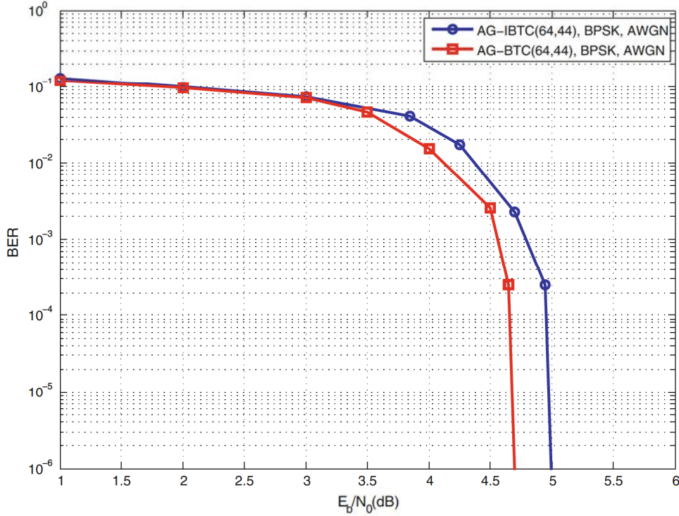
Fig. 5.6 BER of AG-IBTC(64, 44) versus AG-BTC(64, 44) using BPSK over AWGN
