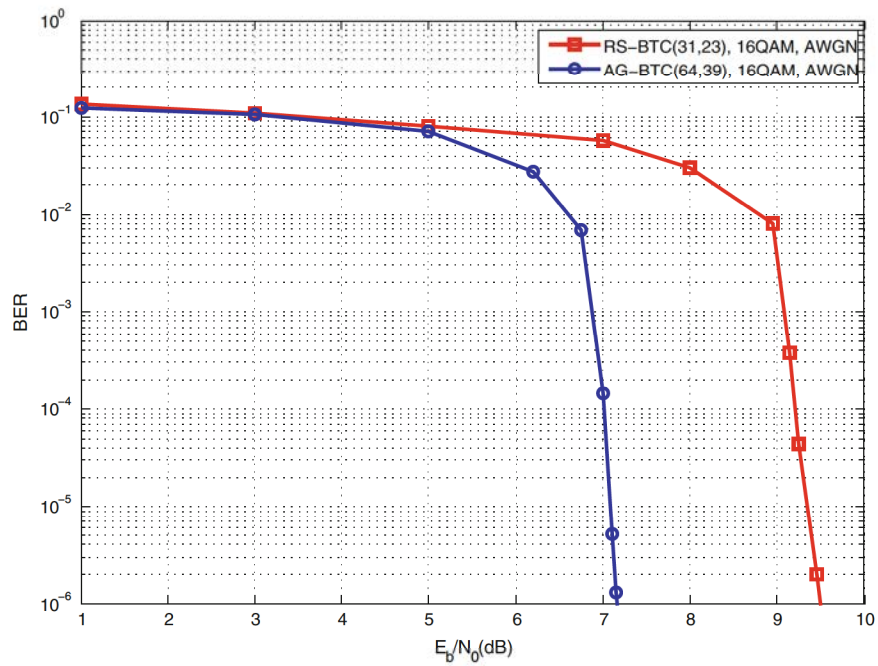
Fig. 4.12 BER of AG-BTC(64,39) versus RS-BTC(31,23) using 16QAM over AWGN
