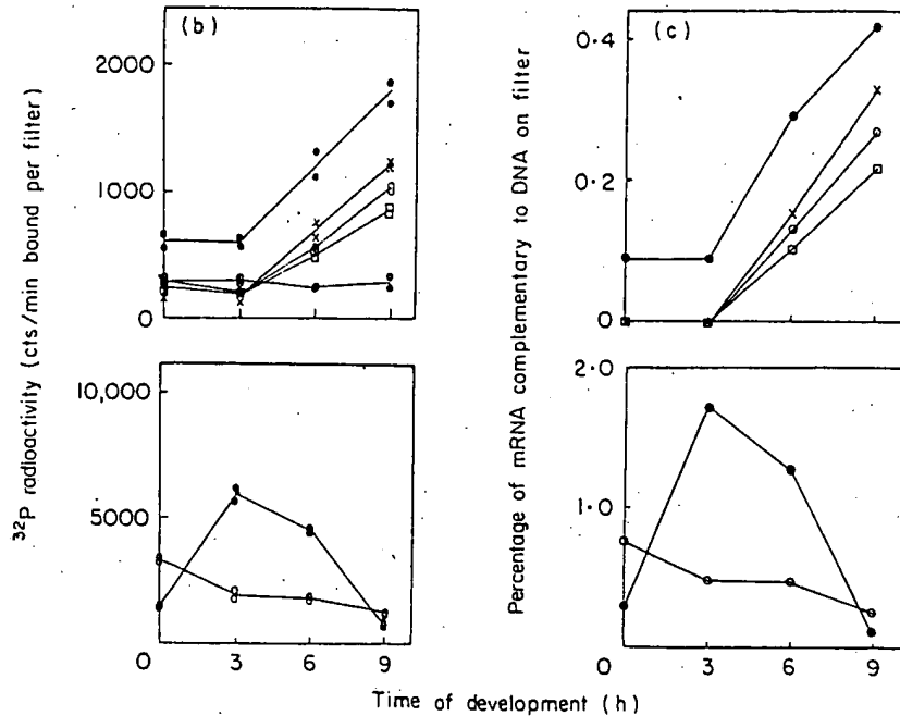
FIG. 2. Developmental time course of changes in concentration of the poly(A)+ RNA complementary to DNA isolated from selected clones.
