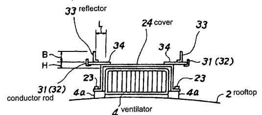
View showing antenna mounting state FIG. 4
