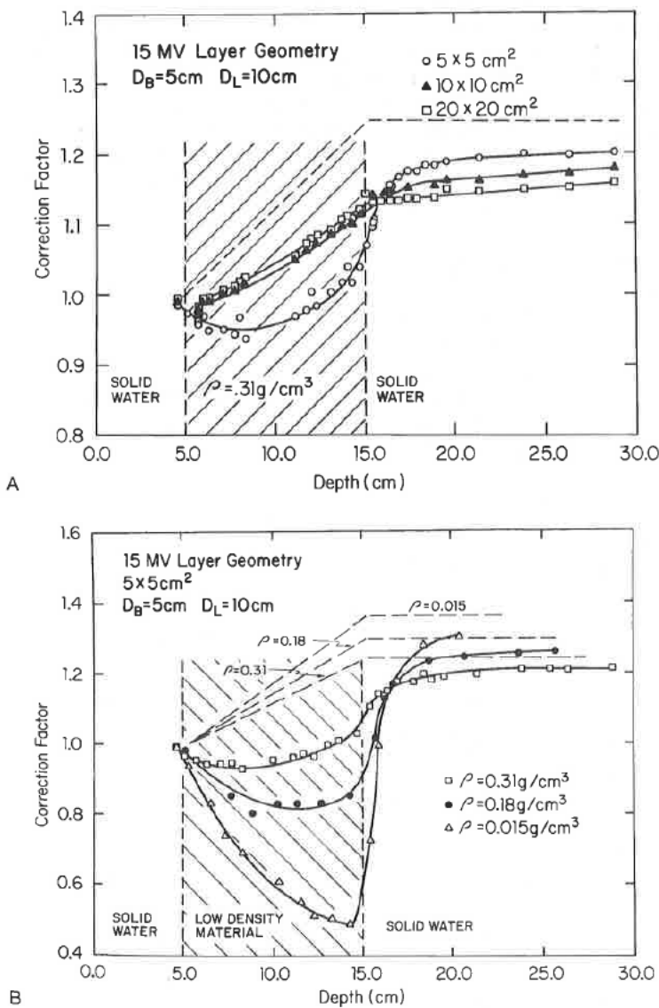
FIGURE 9-6. Dose perturbation factor at tissue-lung interface for 15-MV x-rays: (A) for varying field size and (B) for varying lung density. (Rice RK, Mijnheer BJ, Chin LM: Benchmark measurements for lung dose corrections for x-ray beams. Int J Radiat Oncol Biol Phys 15:399-409, 1988)
