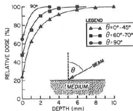
FIGURE 9-3. The variation of surface dose and depth of maximum dose as a function of the angle of incidence of the x-ray beam with the surface (4 MV, 10 × 10 cm).
