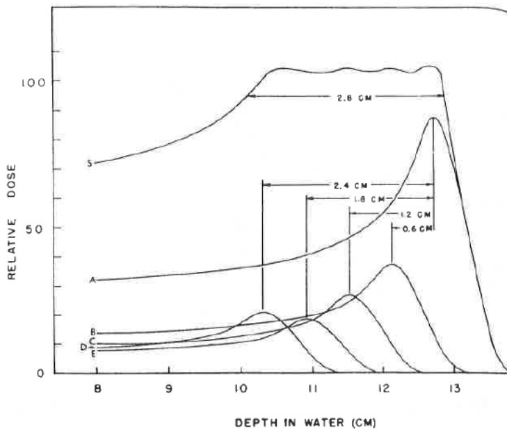
FIGURE 8-24. Drawing illustrating the way in which the Bragg peak for a proton beam can be spread out. Curve A is the depth-dose distribution for the primary beam of 160-MeV protons at the Harvard cyclotron. Beams of lower intensity and shorter range, as illustrated by curves B, C, D, and E, can be added to give a composite curve S, which results in a uniform dose over 2.8 cm. (Hall EJ: Radiobiology for the Radiologist, ed 4. Philadelphia, JB Lippincott, 1994)
