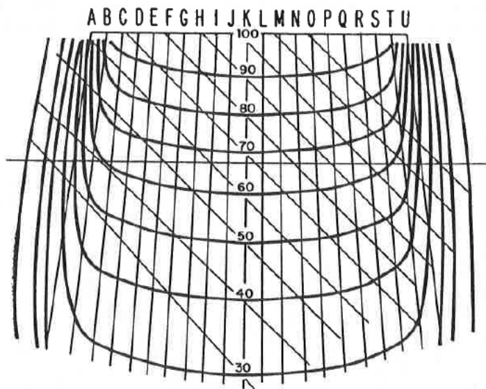
Transmission Ratios for the Construction of Wedge Filter
