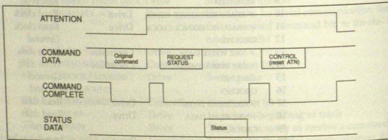
Figure 2.11 Normal command sequence.
