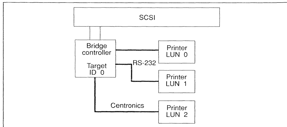
Figure 9.2 Bridge controller with logical units.
