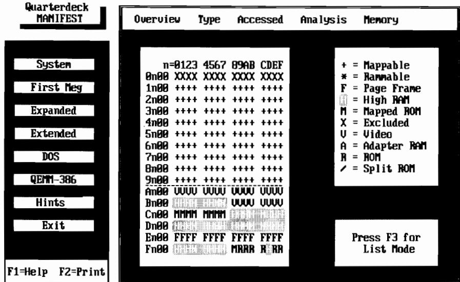
Figure 18-1: One of Manifest's diagnostic screens. The large chart in the center of the screen shows the first 1MB of memory addresses. The top ten rows (0000 through 9000) represent 640K of conventional memory. The next six rows (A000 through F000) represent the 384K of memory addresses between 640K and 1MB. By filling the space with different letters, Manifest shows how these addresses are being used. Some of the memory above 640K is being used by a video adapter board (V) and a ROM BIOS chip (R). In addition, QEMM has added a Page Frame (F) and moved some extended memory to create High RAM (the reversed H's). By counting the H's (each of which represents 4K), we can see that QEMM has made an additional 164K of High RAM available. Some DOS programs can be loaded into this area, conserving the lower 640K.
