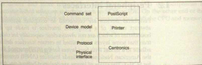
Figure 1.2 Layers of a printer interface.
