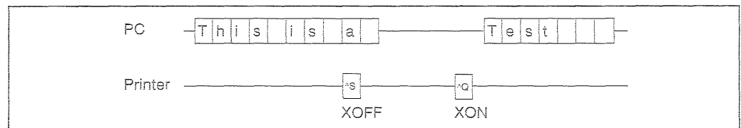
Figure 2.2 XON/XOFF protocol.
