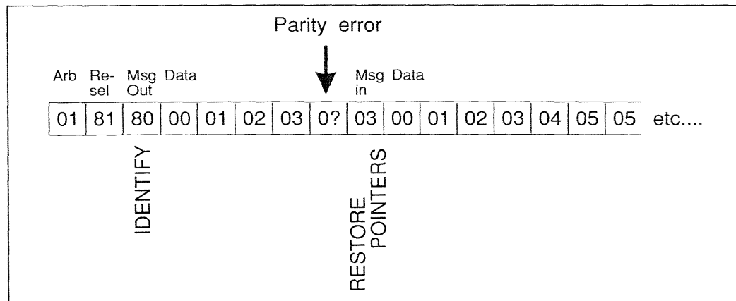
Figure 11.1 Parity error.
