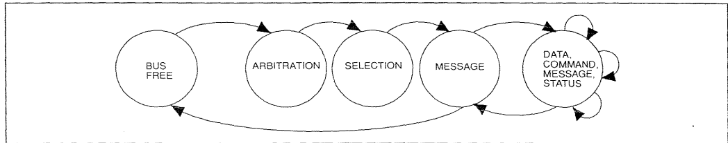
Figure 10.11 Simplified SCSI phase diagram.
