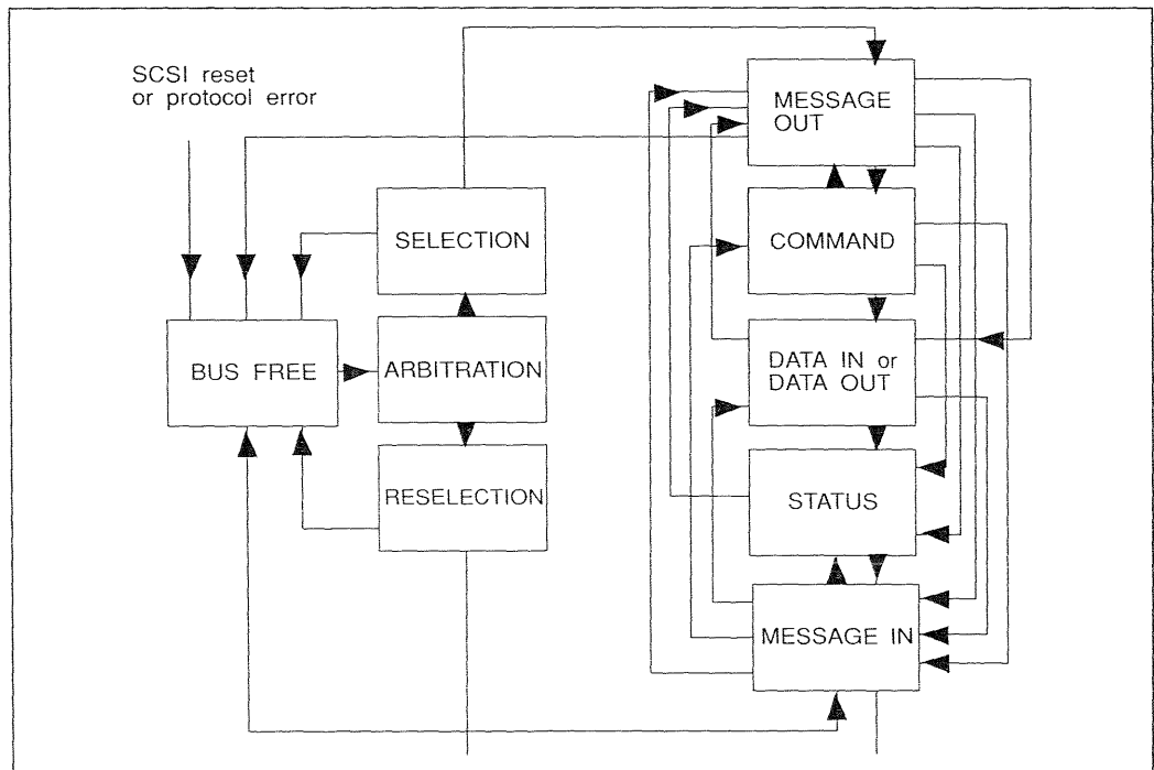
Figure 10.12 Complete SCSI phase diagram.
