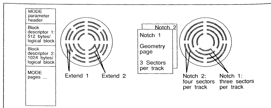
Figure 13.2 SCSI extends and notches.
