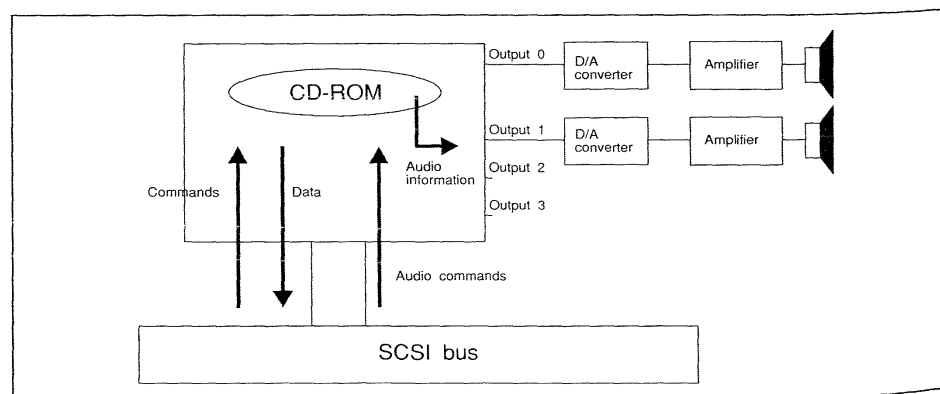
Figure 20.1 Model of a CD-ROM drive.
