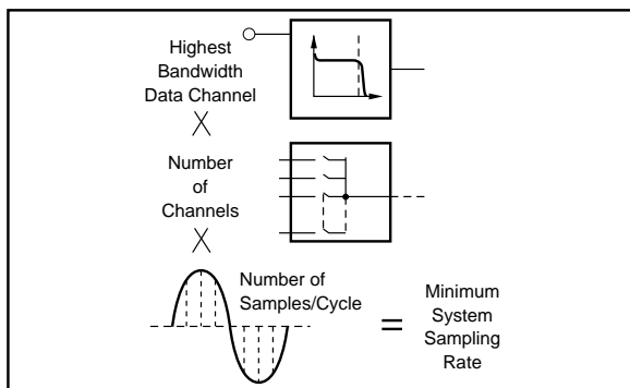
FIGURE 1. Determining Minimum System Sampling Rate.
