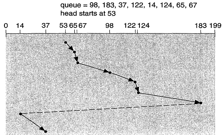
Figure 12.5 C-LOOK disk scheduling.
