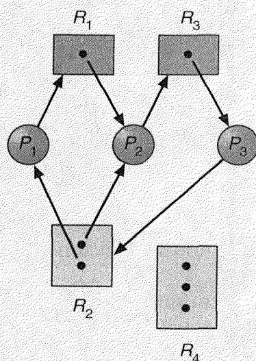
Figure 7.2 Resource-allocation graph with a deadlock.
