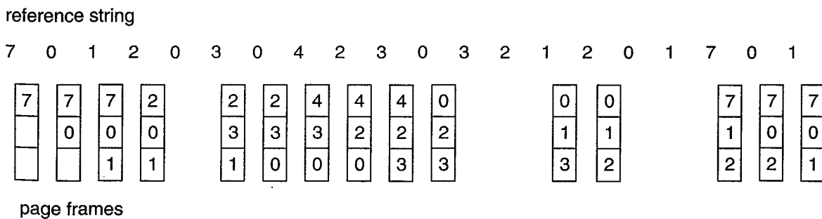
Figure 9.8 FIFO page-replacement algorithm.
