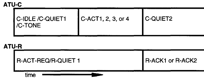
Figure 30 – Timing diagram of activation and acknowledgment (12.2-12.3)
