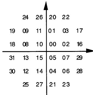
Figure 16 – Constellation labels for b = 5
