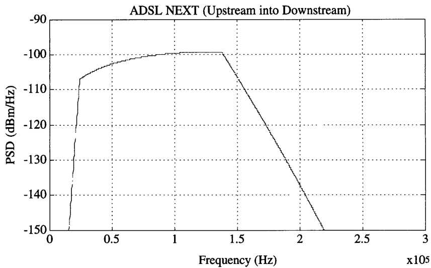
Figure B.5 – Theoretical 10-disturber ADSL NEXT
