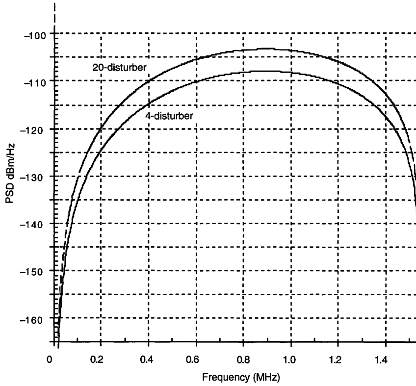
Figure B.3 – 4 and 20-disturber T1 NEXT
