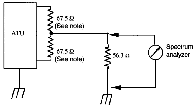
Figure 25 – Measurement method for longitudinal output voltage
