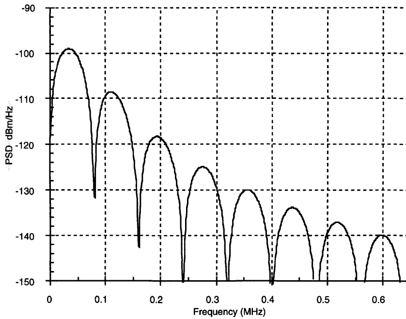
Figure B.1 – 24-disturber DSL NEXT
