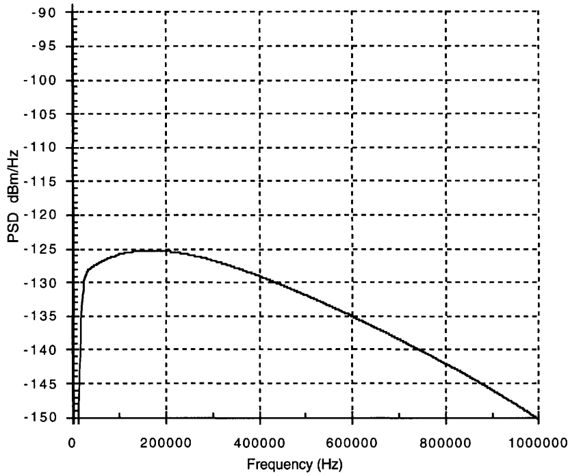
Figure B.4 – Theoretical 10-disturber ADSL FEXT
