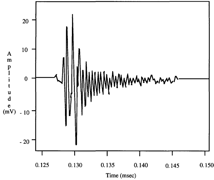
Figure 39 – Test impulse #1
