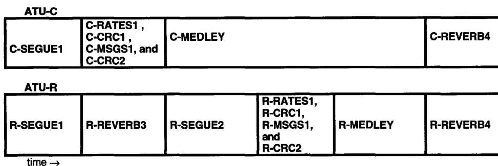
Figure 32 – Timing diagram of channel analysis (12.6-12.7)
