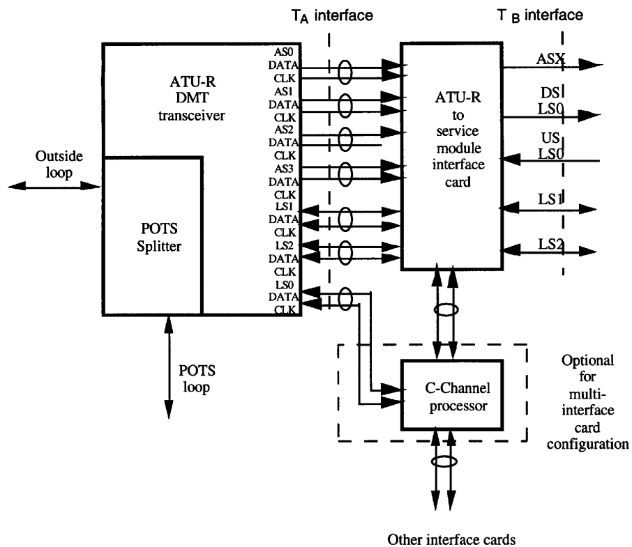
Figure 23 – ADSL entrance unit block diagram
