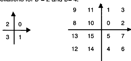
Figure 14 – Constellation labels for b = 2 and b = 4
