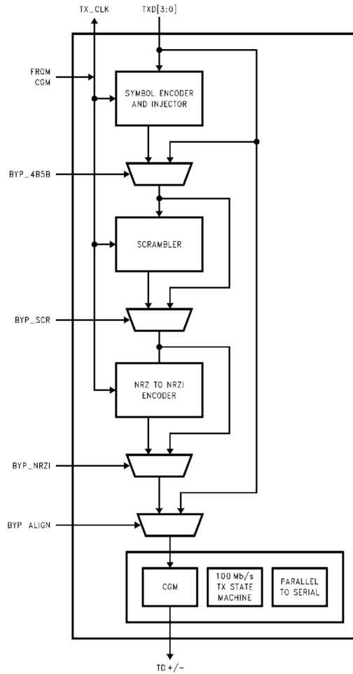
FIGURE 4. 100BASE-X Transmitter
