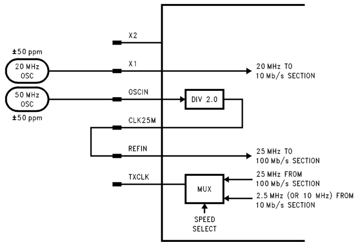
FIGURE 7. 50 MHz and 20 MHz Reference
