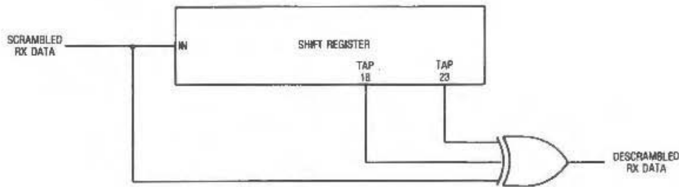
Fig 11-12 Descrambler
