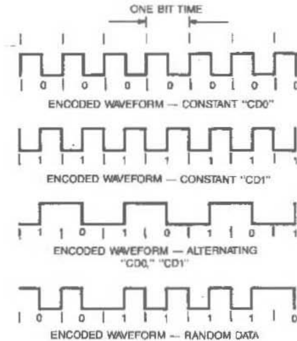
Fig 12-10 Examples of Manchester Waveforms
