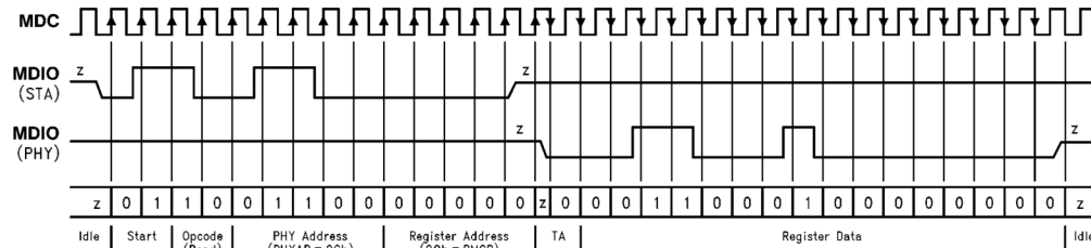
FIGURE 2. Typical MDC/MDIO Read Operation
