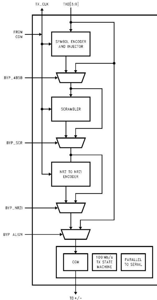
FIGURE 4. 100BASE-X Transmitter
