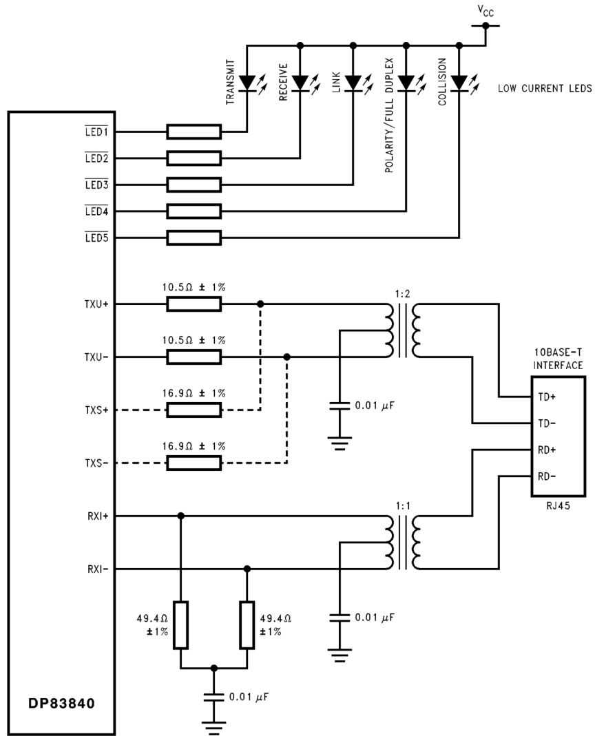
FIGURE 12. Typical 10BASE-T (UTP) Node Application
