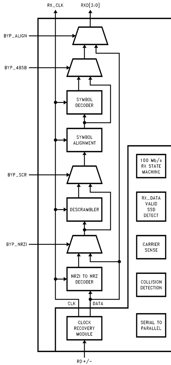
FIGURE 5. 100BASE-X Receiver
