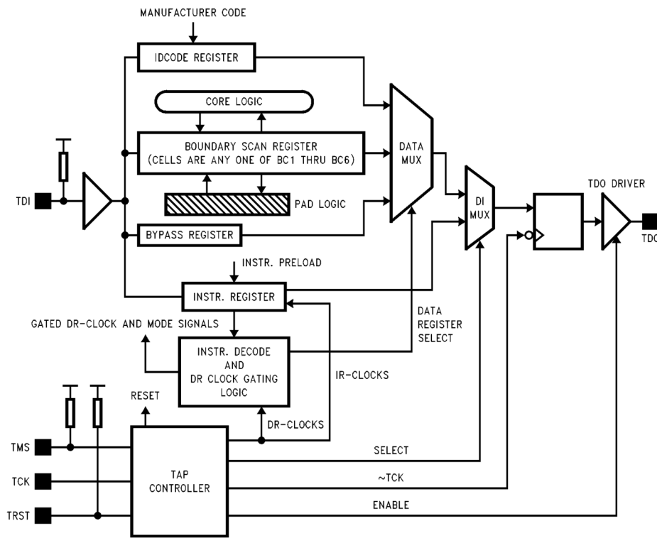
FIGURE 13. IEEE 1149.1 Architecture
