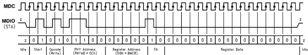
FIGURE 3. Typical MDC/MDIO Write Operation
