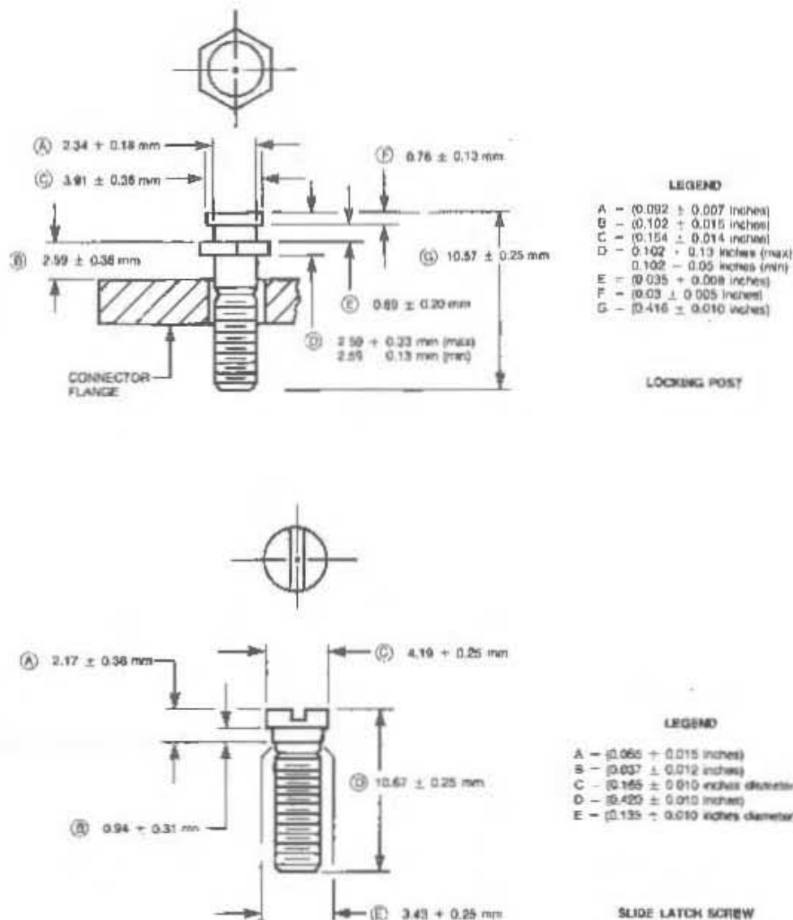
Fig 7-18 Connector Locking Posts
