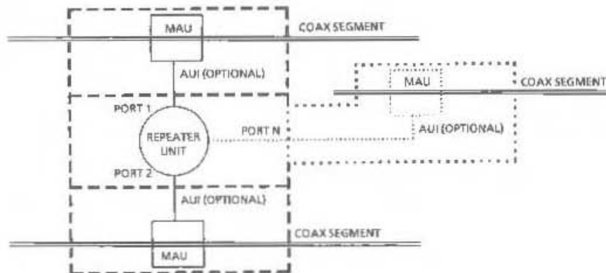
Fig 9-1 Repeater Set, Coax-to-Coax Configuration
