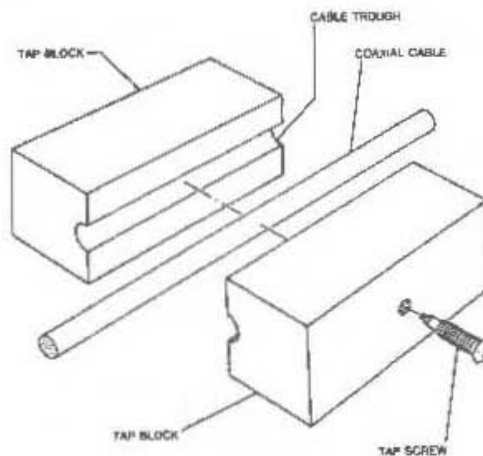
Fig 8-8 Coaxial Tap Connector Configuration Concepts
