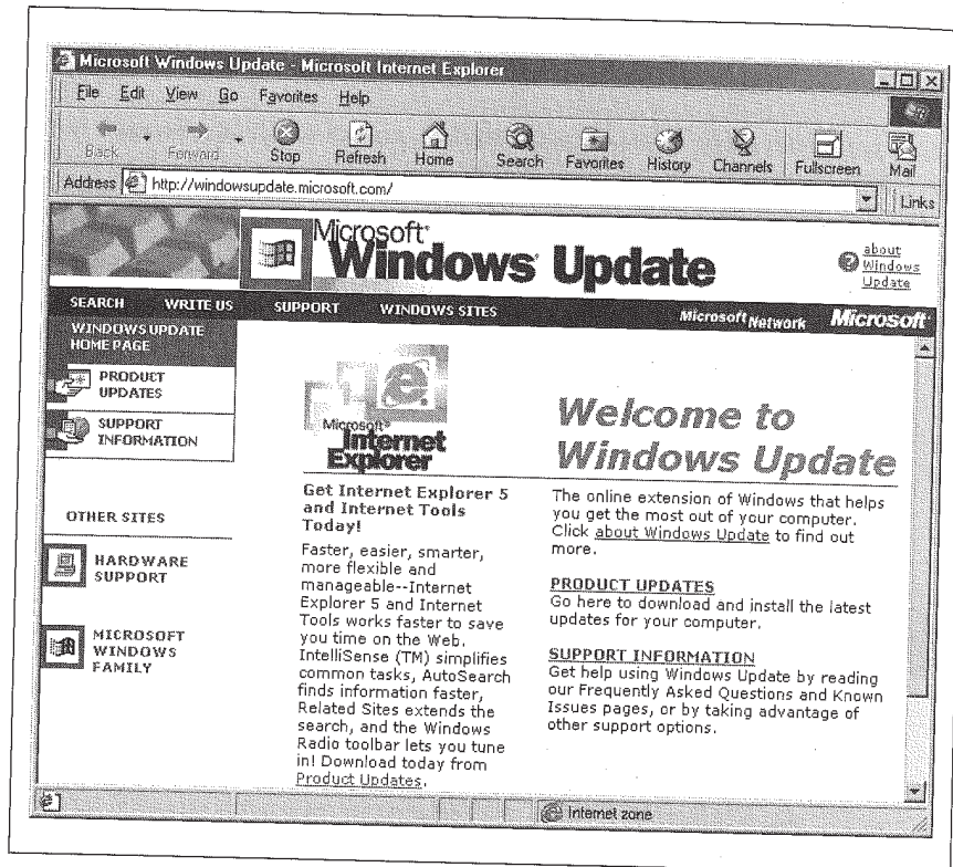
Figure 4-29: Windows Update
