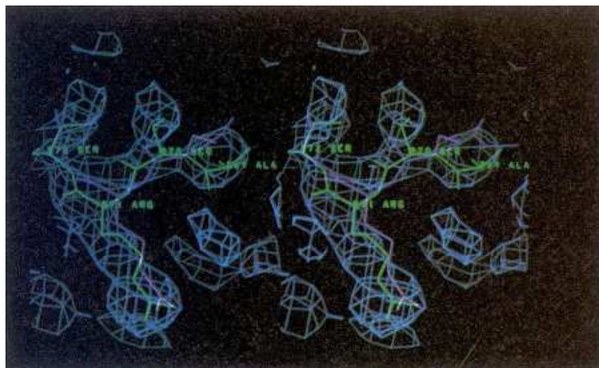
Fig. 4 Stereo image of the electron density map ( 2F_b - F_c , R = 0.35 ) of the neuraminidase loop 368-372 in the complex with NC41 Fab. Residues here are labelled 868-872. The yellow model shows the current fit of the loop in the complex structure. The purple model is the position of this loop in uncomplexed N9 neuraminidase.
