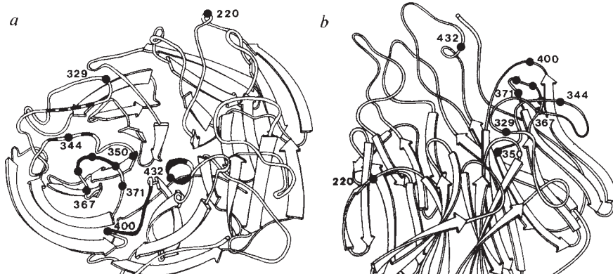
Fig. 1 Schematic diagrams of chain fold in N2 and N9 neuraminidase viewed down the 4-fold axis (a) and perpendicular to this axis (b). The symmetry axis is bottom right in a and standing vertical at the left rear in b. The view of the neuraminidase in b is similar to that shown in Fig. 5. Tagged residues and adjacent chain segments are referred to in the text. N2 numbering is used. In a, the side chains of amino acids 368-370 point towards the viewer, whilst that of Arg 371 points away and into the catalytic site located above and to the right of C α 371. Mutations at positions 367, 369, 370, 400, and 432, as detailed in Fig. 2, abolish the binding of NC41 antibody to neuraminidase, whereas mutations at 368 and 329 reduce that binding. A mutation at 220, which falls outside the NC41 epitope, has no effect on NC41 binding to neuraminidase (see Fig. 2). In a, solid chain segments show regions in contact with the NC41 antibody: contact assignments in the
