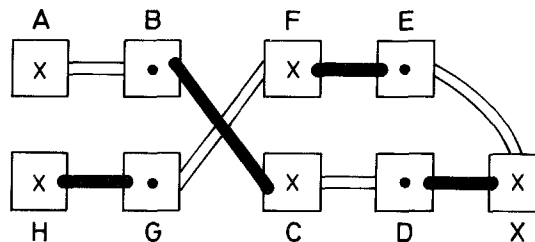
Fig. 2 Schematic drawing of the strand topology in a V-domain viewed parallel to the strands.
