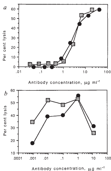
Fig. 5 a , Complement lysis and b , ADCC of the reshaped human (□) and rat YTH 34.5HL (●) antibodies. Antibody HuVHCAMP (Ser27 → Phe, Thr30 → Ser)-Hu1GG1, HuVLCAMP-Hu1GK was purified from supernatants of cells in stationary phase by affinity chromatography on protein-A Sepharose. The yield (about 10 mg l -1 ) was measured spectrophotometrically. Complement and ADCC assays were performed as in Fig. 4.
