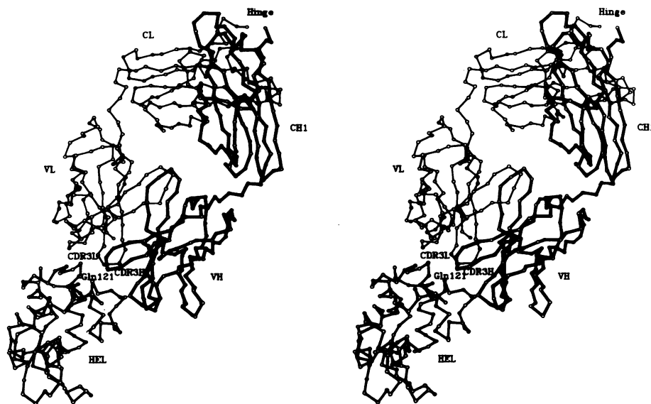
Fig. 1. Stereo diagram of the C\alpha skeleton of the complex. Fab is shown (upper right) with the heavy and light chains with thick and thin bonds, respectively. The lysozyme active site is the cleft containing the label HEL. Antibody-antigen interactions are most numerous between lysozyme and the heavy chain CDR loops.
