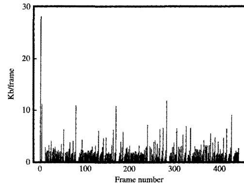
Figure 3 Illustration of Bamba video compression with dynamic-frame-rate-control algorithm. The number of bits transmitted is shown for each frame of a sample video sequence.
