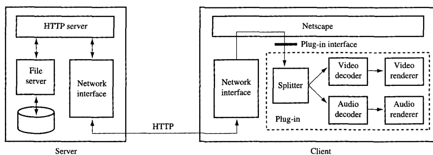
Figure 1. Bamba system block diagram.
