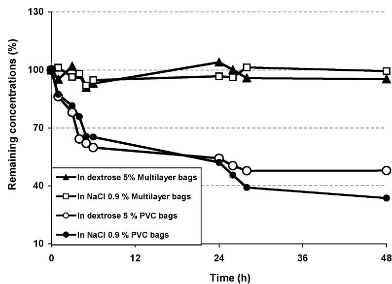
Fig. 3. Remaining concentrations of diazepam after storage in multilayer or PVC bags.
