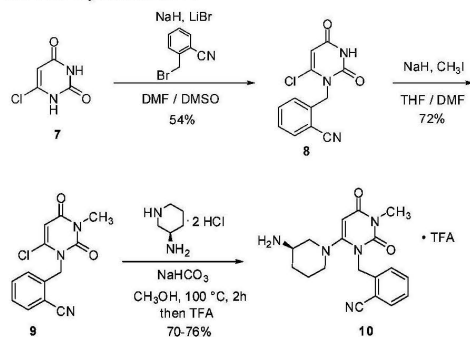
Scheme 2. Synthesis of 10
