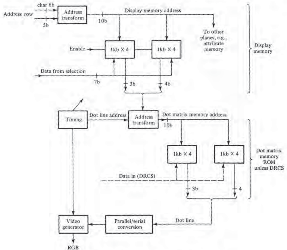
Figure 9.5 Structure of display and dot matrix memories.
