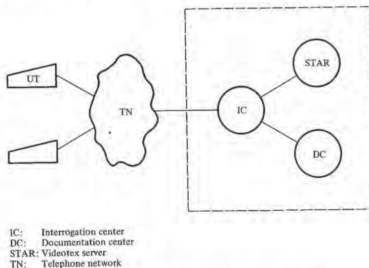
Figure 12.8 French Electronic Directory system components.
