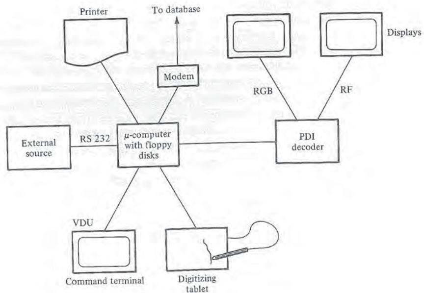
Figure 9.11 VIPS hardware configuration
