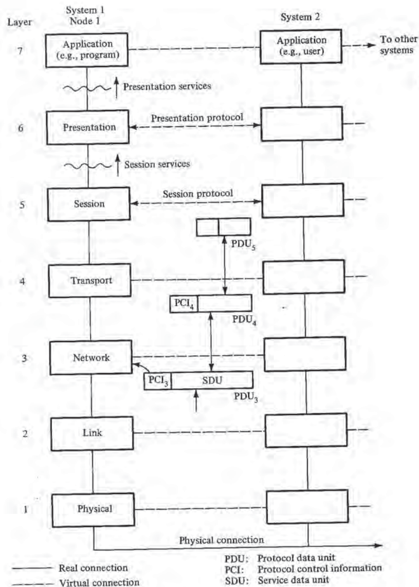
Figure 3.1 ISO Open Systems Interconnection reference model.
