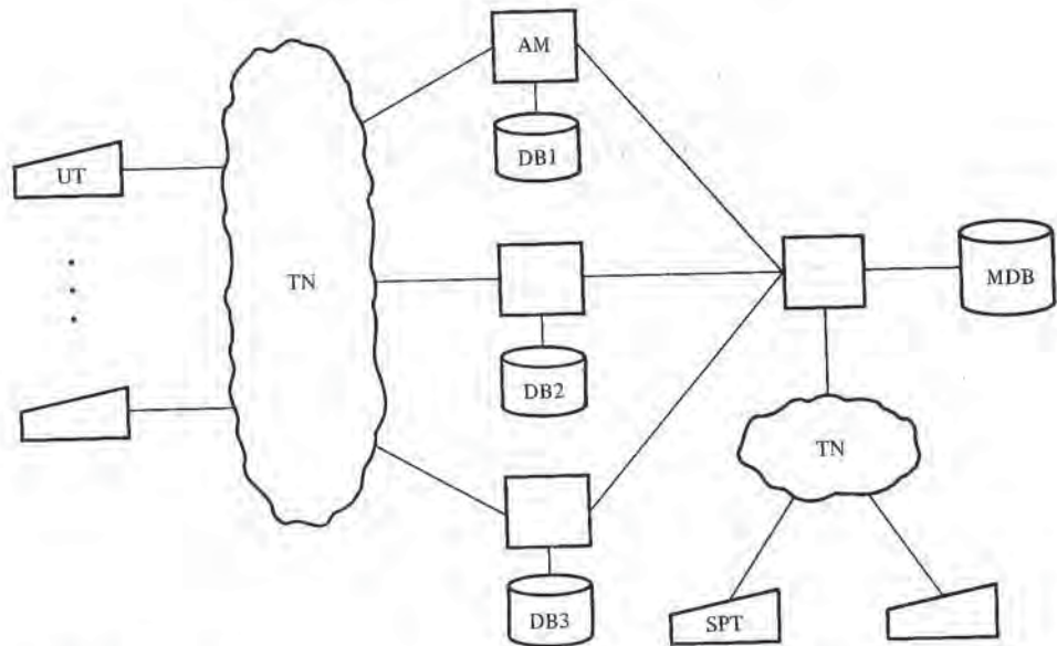
Figure 6.5 Replicated databases.
