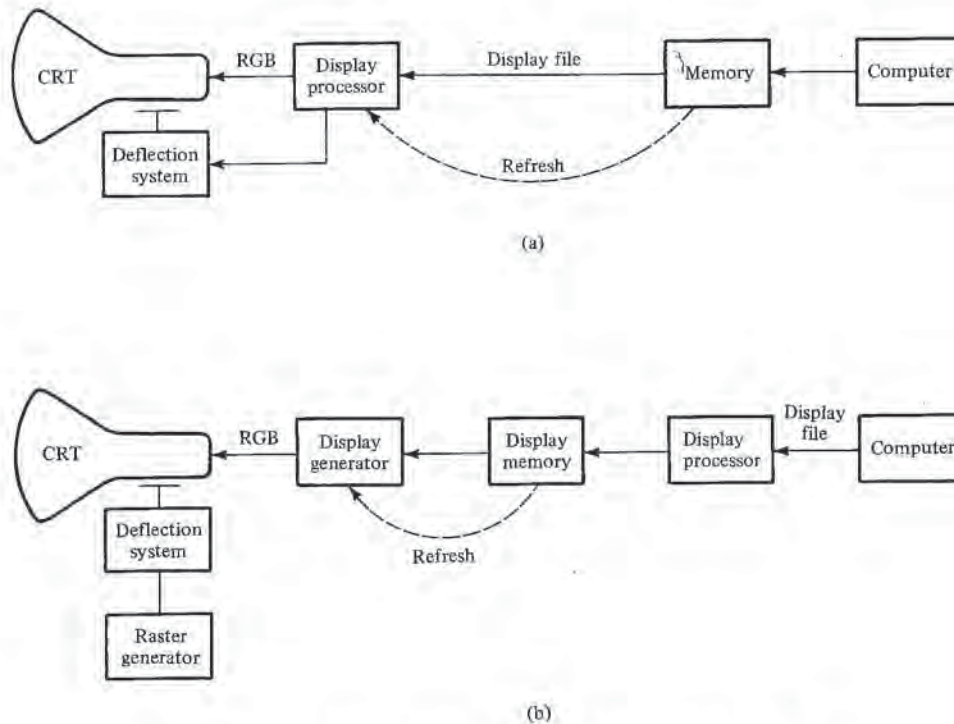
Figure 8.3 Principle of graphic systems: (a) random deflection; (b) raster scan.
