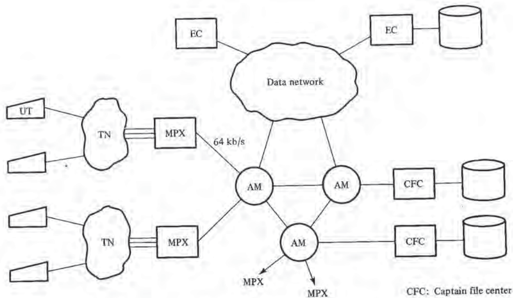
Figure 6.14 Captain network.
