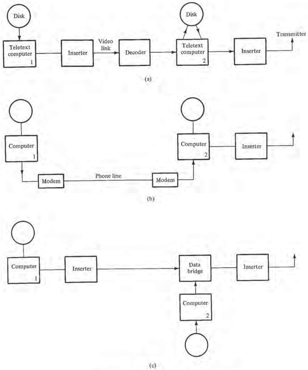
Figure 12.11 Possibilities for linking two teletext systems.
