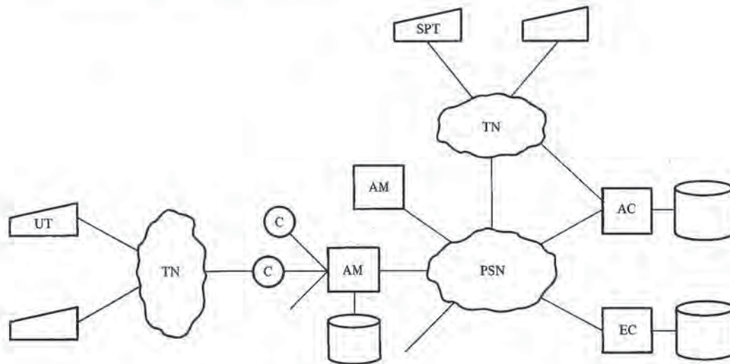
Figure 6.7 System with two levels of concentration.
