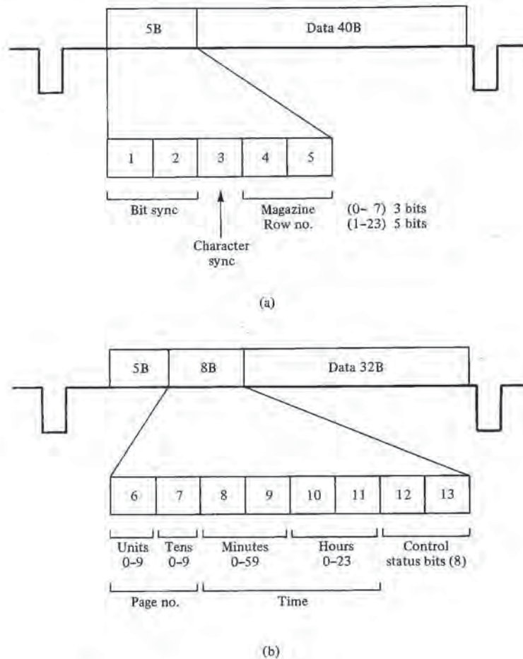
Figure 5.2 U.K. teletext data lines: (a) rows 1–23; (b) row 0.
