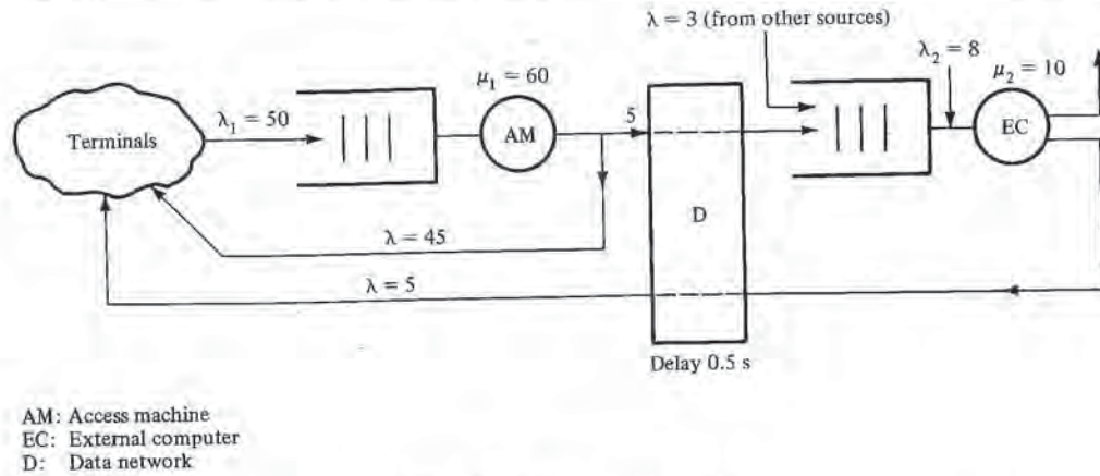
Figure 15.5 Multistage open system.
