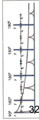
Fig. 9—The schematic is of Carr-Purcell-Meiboom-Gill pulse-echo sequence.
