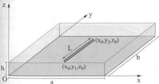
Fig. 1. Horizontal hole layout in the reservoir.
