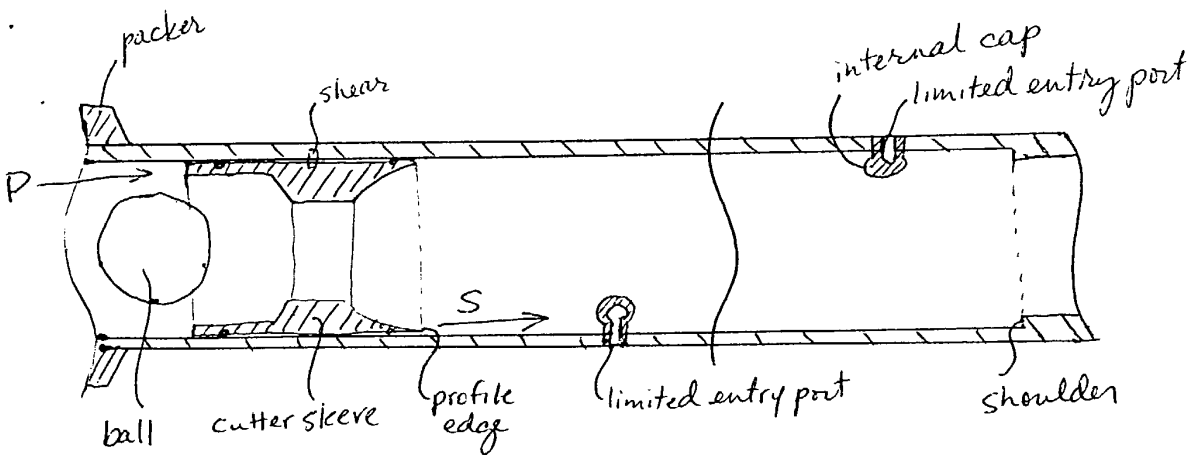
stage 2 tubing in cross section
