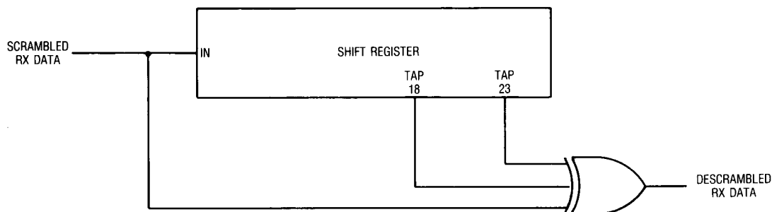
Figure 11–12—Descrambler
