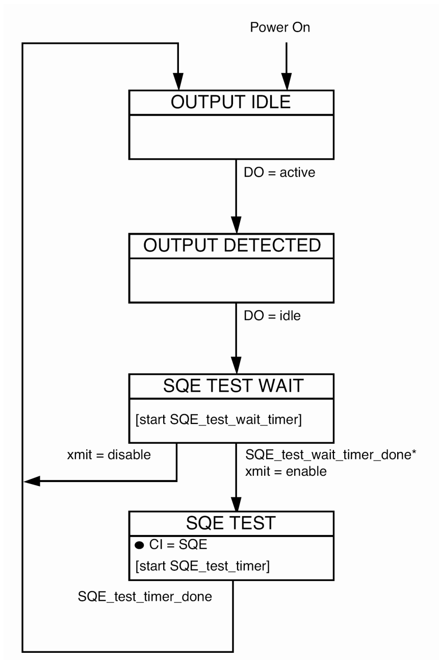
Figure 18–2— signal_quality_error Message Test function state diagram
