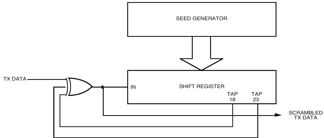
Figure 11–10—Scrambler
