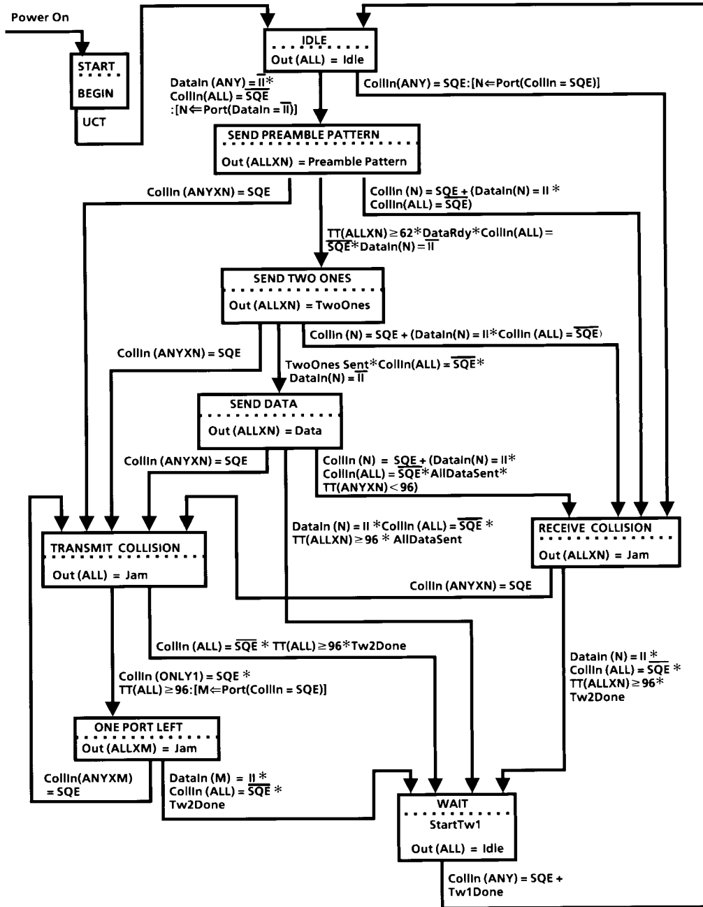
Figure 9-2—Repeater unit state diagram
