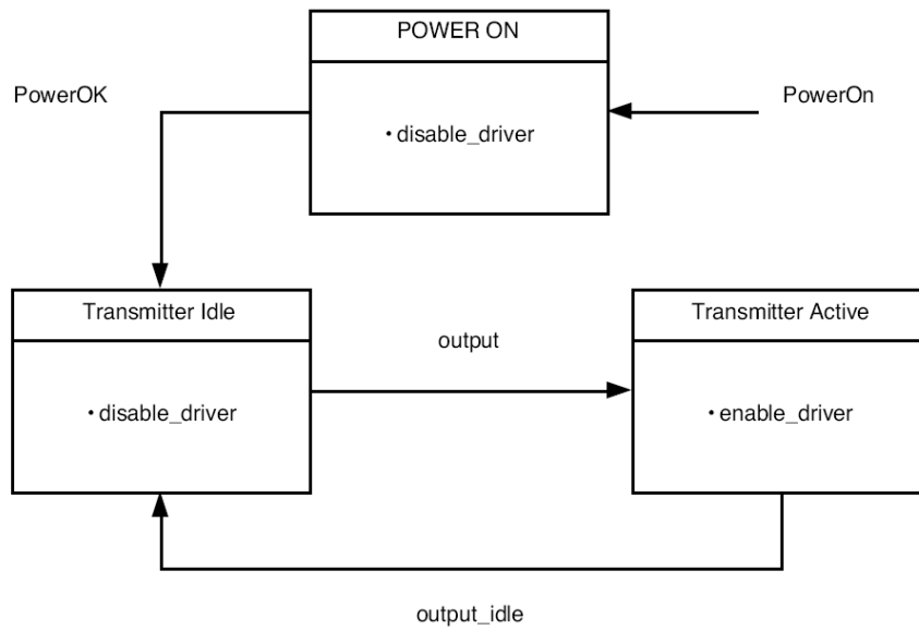
c) Transmit function state diagram
