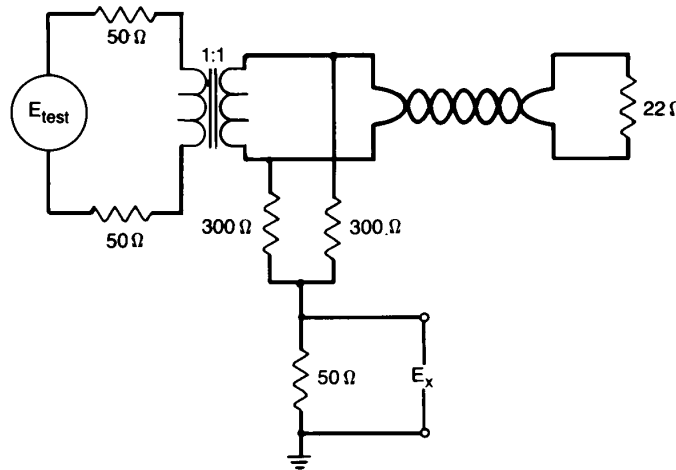
Figure 12–32—Cable balance test
