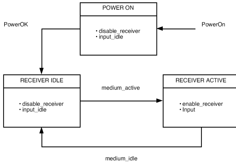
b) Collision Presence function state diagram
