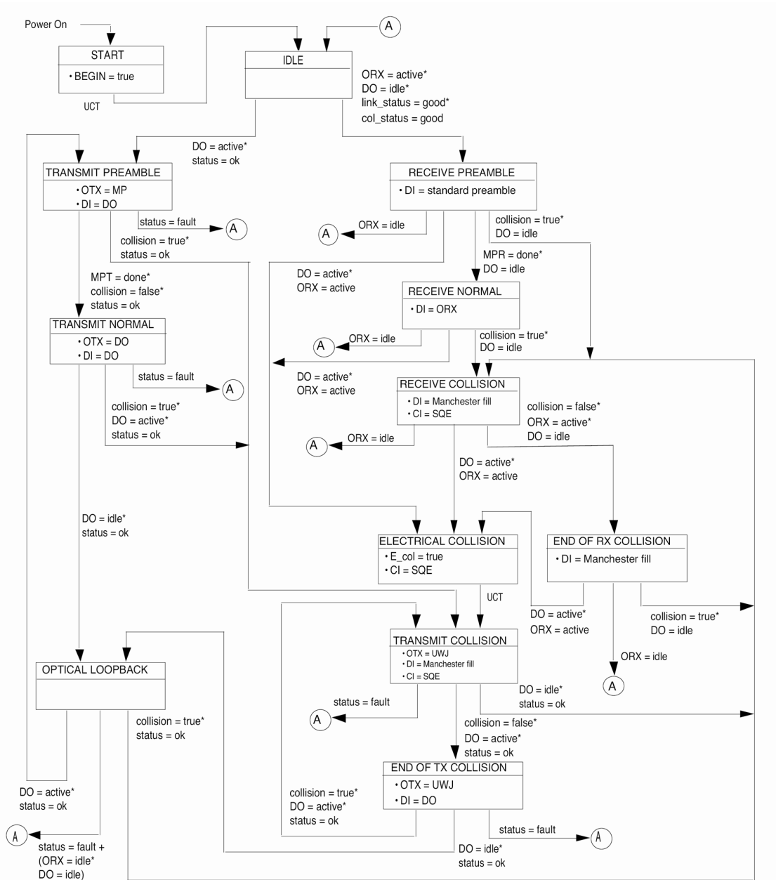
Figure 16-2—Transmit and Receive function state diagram
