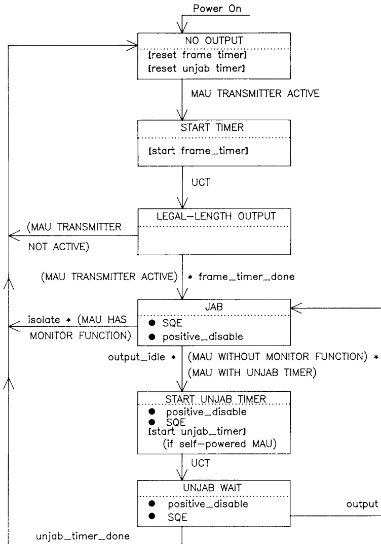
Figure 8-4—Jabber function
