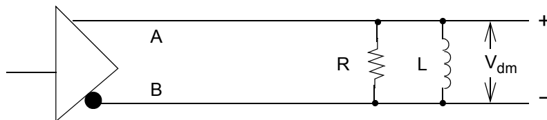
Figure 7-11—Differential output voltage, loaded
