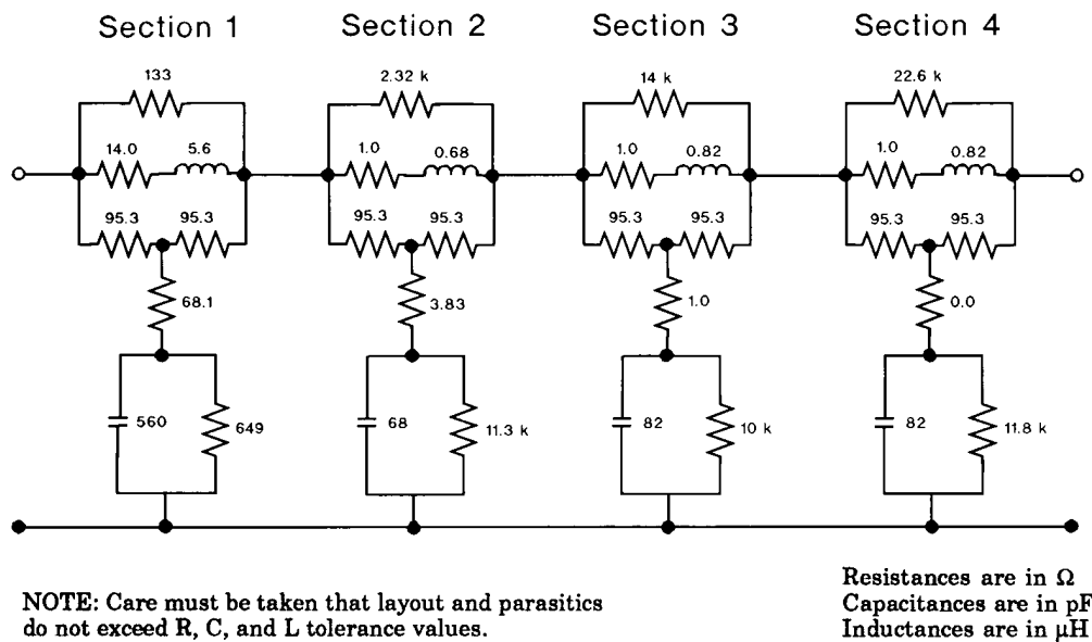
Figure 14–7—Twisted-pair model for 10BASE-T
