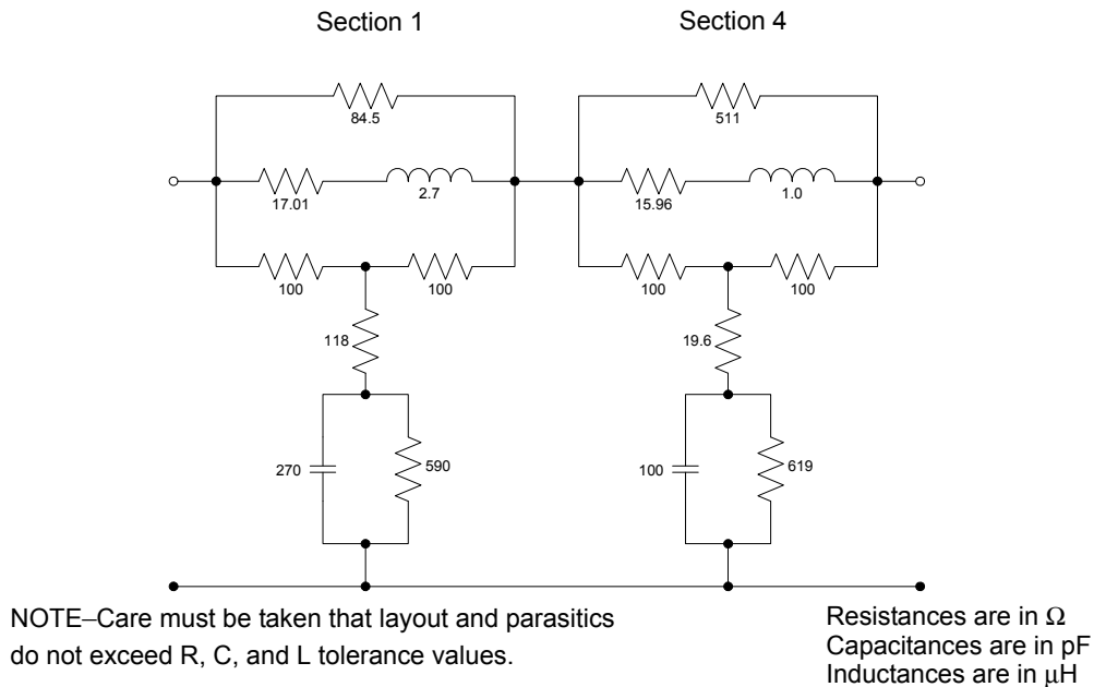
Figure 14–8—Twisted-pair model for 10BASE-Te
