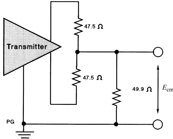
Figure 14-15—Common-mode output voltage test circuit
