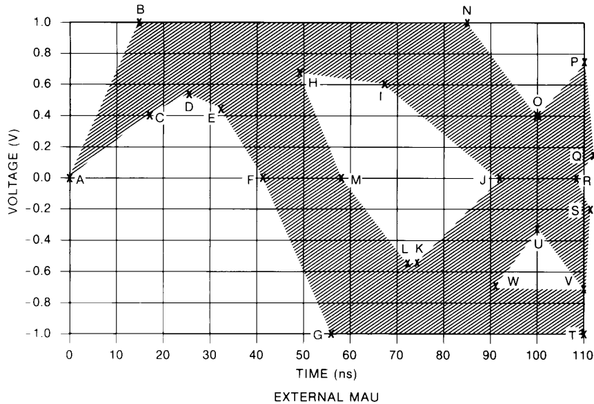
Figure 14-10—Voltage template
