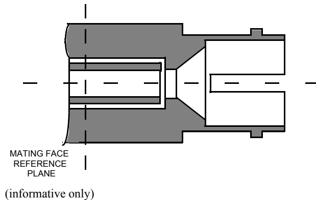
Figure 15-6—BFOC/2.5 connector plug
