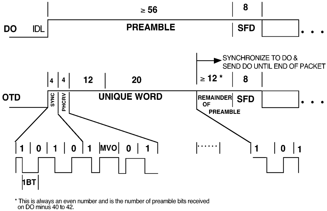
Figure 16–1—10BASE-FP MAU preamble encoding
