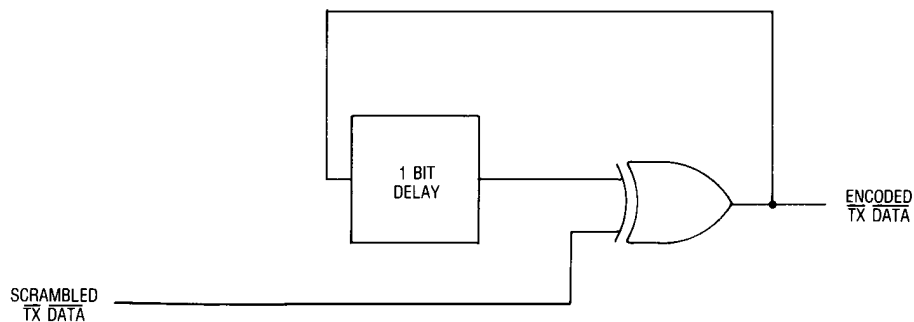
Figure 11–11—Differential encoder
