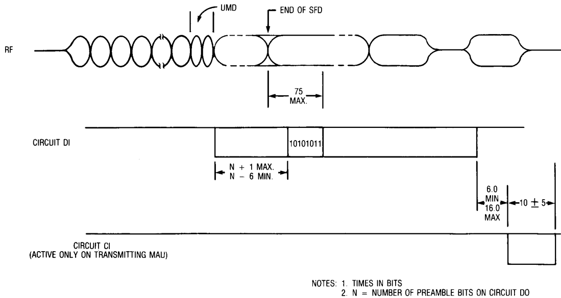
Figure 11–13—No collision timing diagram (coax to AU1)
