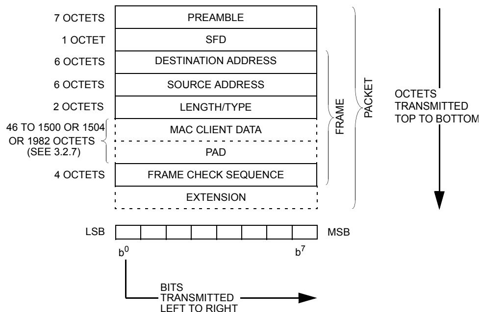
Figure 3–1—Packet format
