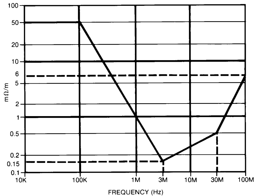
Figure 8–7—Maximum coaxial cable transfer impedance
