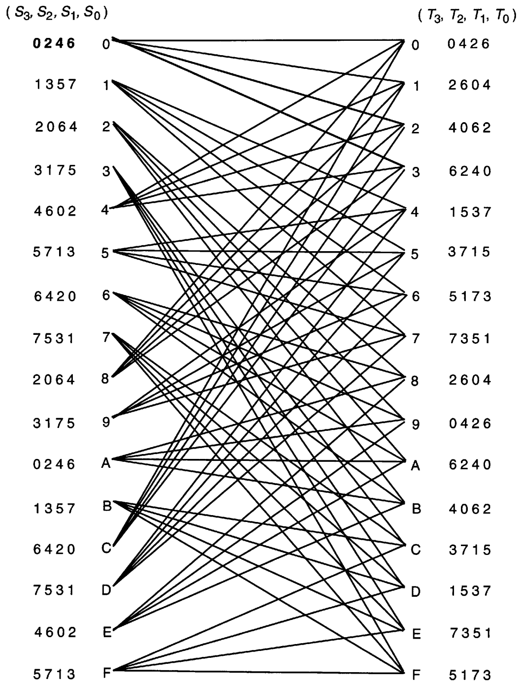
Figure 12 – Trellis diagram
