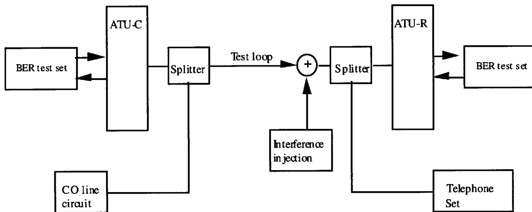
Figure 37 – Overview of test setup
