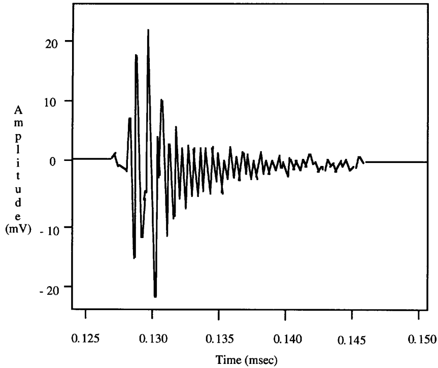
Figure 39 – Test impulse #1
