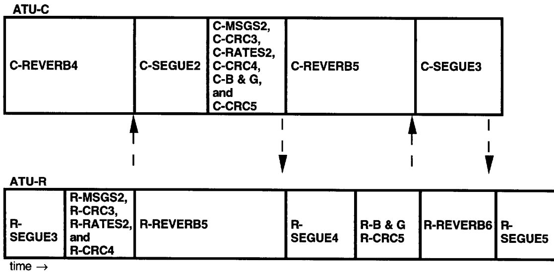
Figure 34 – Timing diagram of exchange (12.8-12.9)
