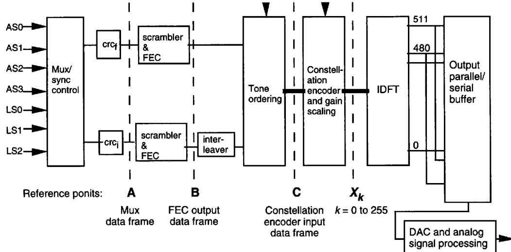
Figure 2 – ATU-C transmitter reference diagram
