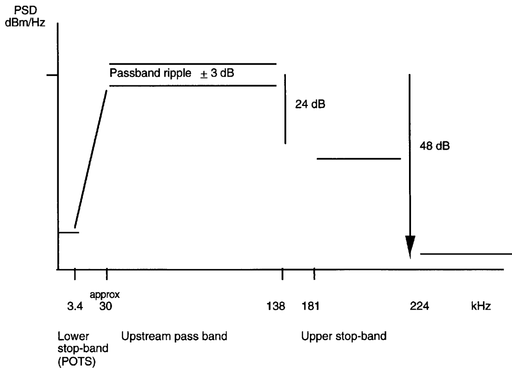
Figure 22 – ATU-R transmitter PSD mask
