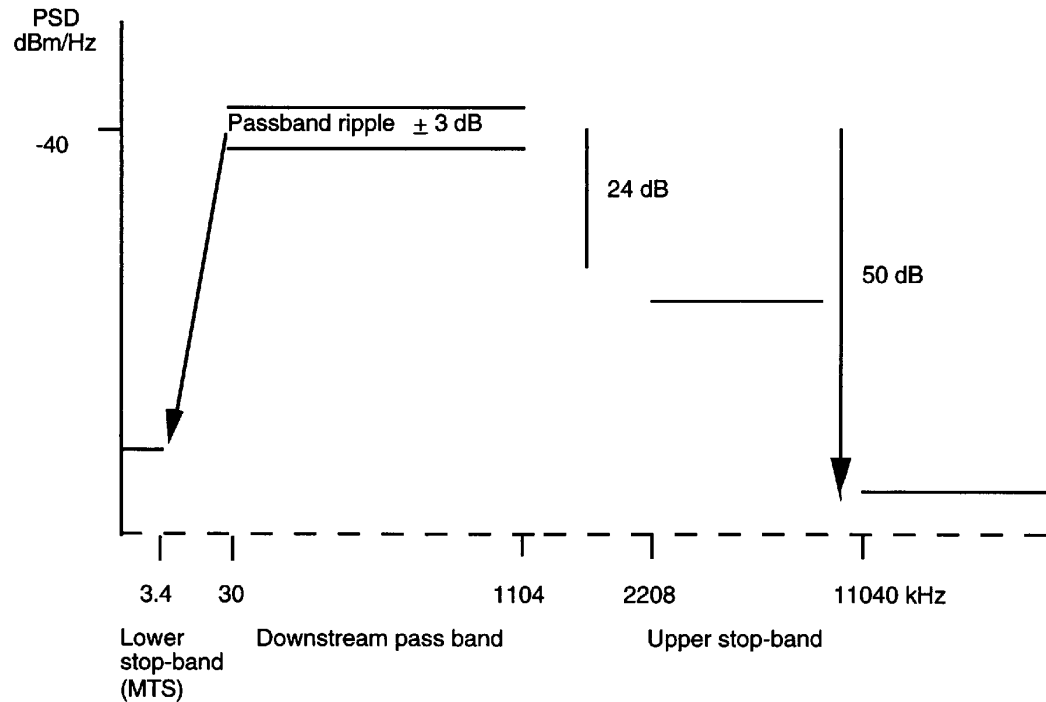
Figure 17 – ATU-C transmitter PSD mask
