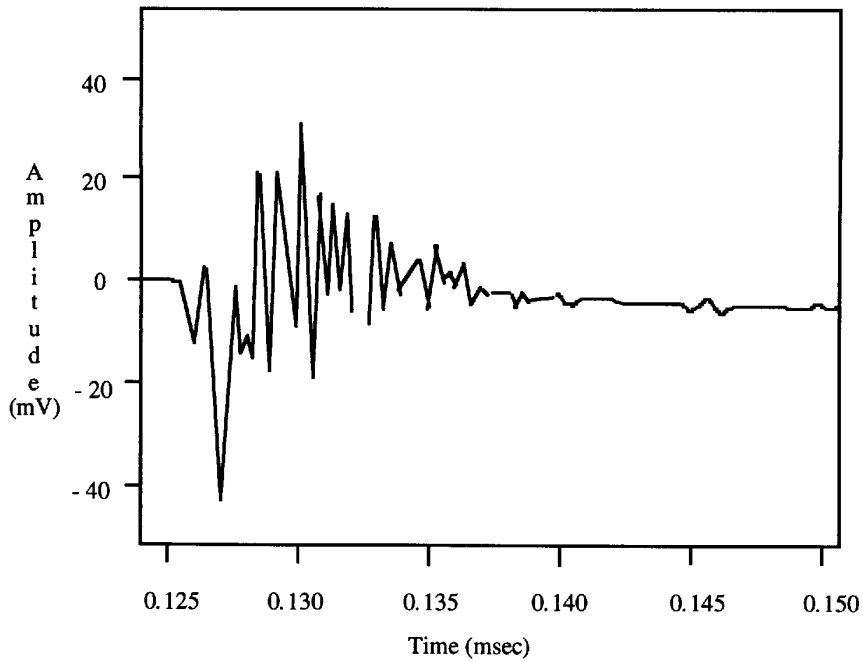
Figure 40 – Test impulse #2
