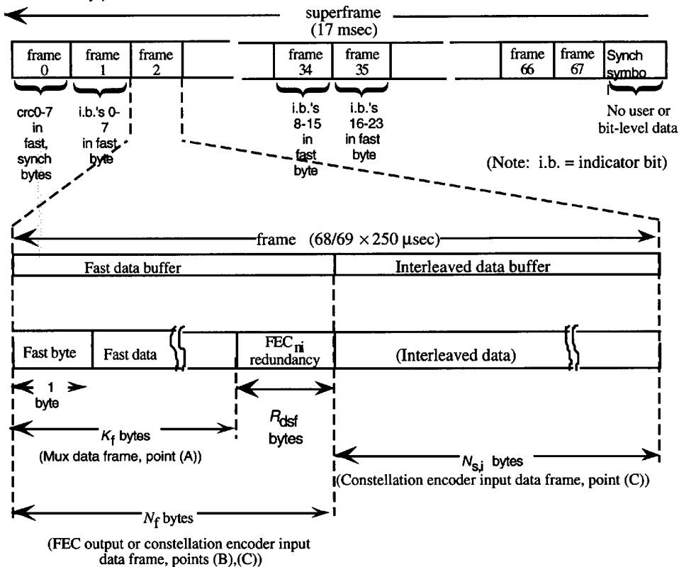
Figure 5 – ADSL superframe structure – ATU-C transmitter
