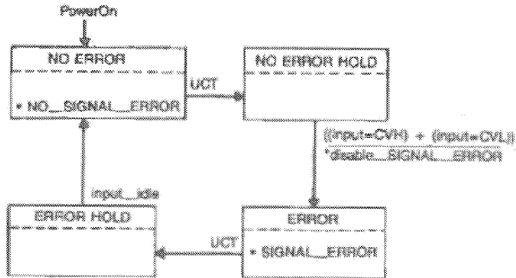
Fig 13-8 DTE PLS Error Sense Function
