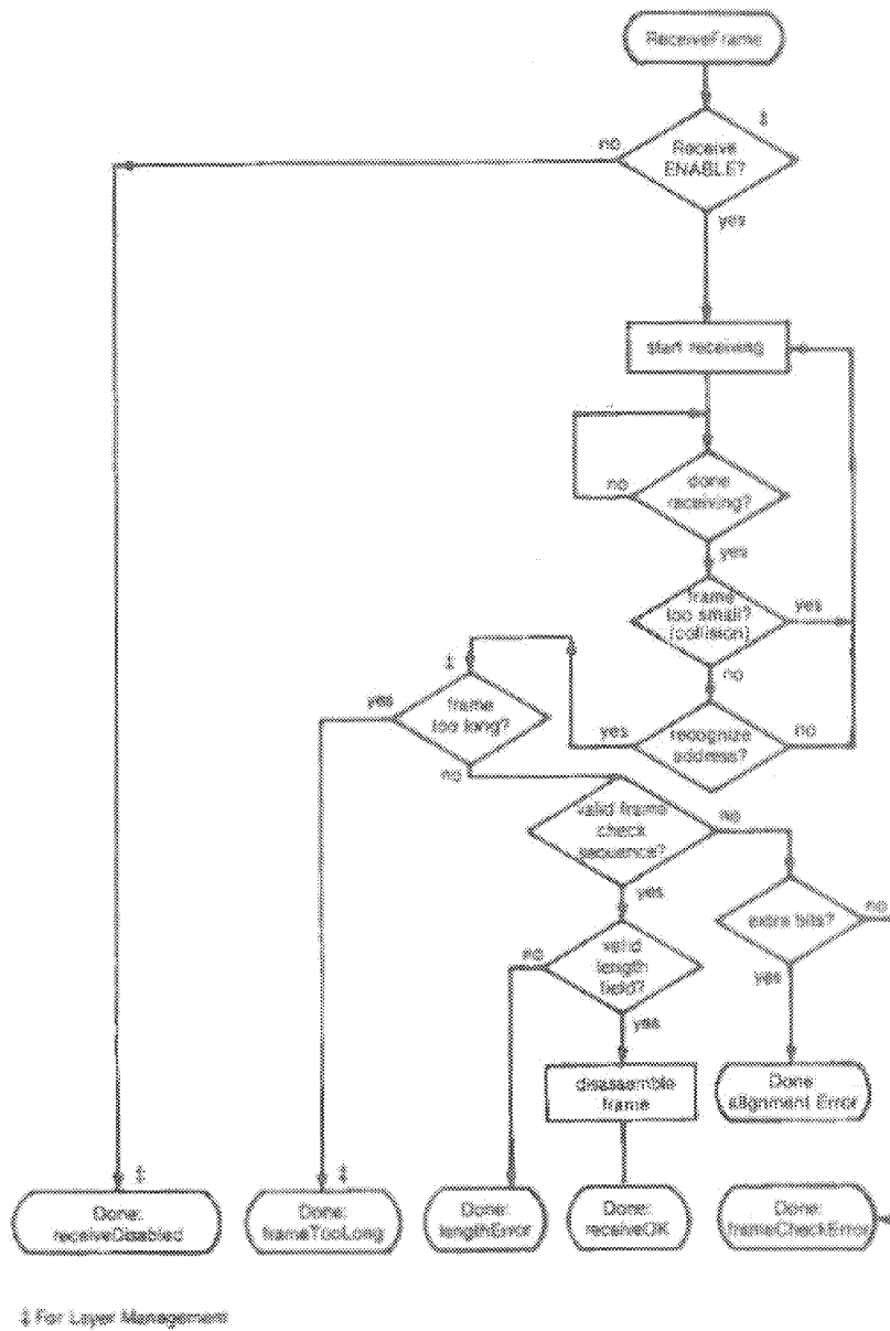
(b) ReceiveFrame
