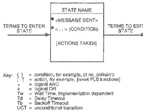
Fig 1-2 State Diagram Notation Example
