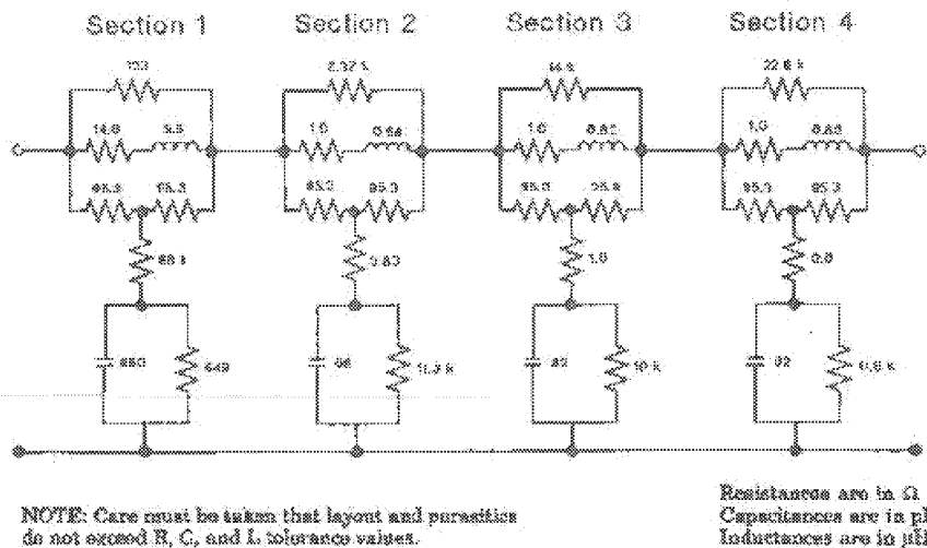
Fig 14-7 Twisted-Pair Model
