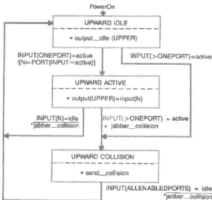
Fig 12-13 Hub PLS Upward Transfer Function
