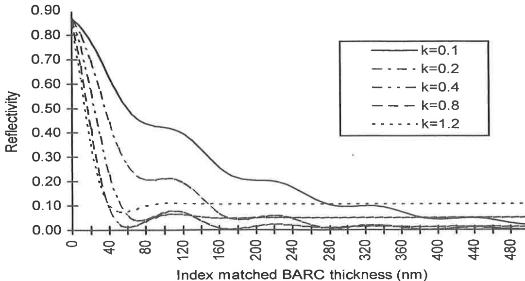
Figure 6 Substrate reflectivity vs. bottom ARC thickness for real index matched materials ( n = 1.7 at 365 nm) and extinction coefficient values from 0.1 to 1.2. The best performance for a thin BARC layer may be possible with k values near 0.8.
