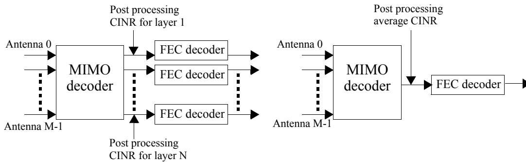
Figure 230a—Post processed CINR for MIMO region
