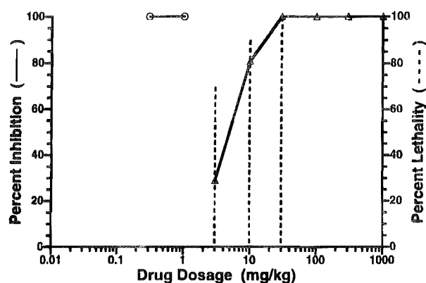
Figure 2. Antitumor activity of LY231514 therapy (i.p., qd \times 10 ) against L5178Y/TK-/HX- lymphoma for mice on low folate diet with no folate supplementation (○) and for mice on low folate diet that received 15 mg/kg/day daily folate supplementation (△). Vertical dashed lines represent percent lethality in mice on low folate diet with no folate supplementation. No lethality was observed in mice that received folate supplementation.
