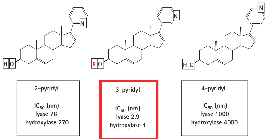
FIG. 2. The structure of abiraterone and abiraterone acetate (centre). The effect variations in the orientation of the pyridyl substituent have on the potency of 17 \alpha -hydroxylase/C 17,20 -lyase inhibition.
