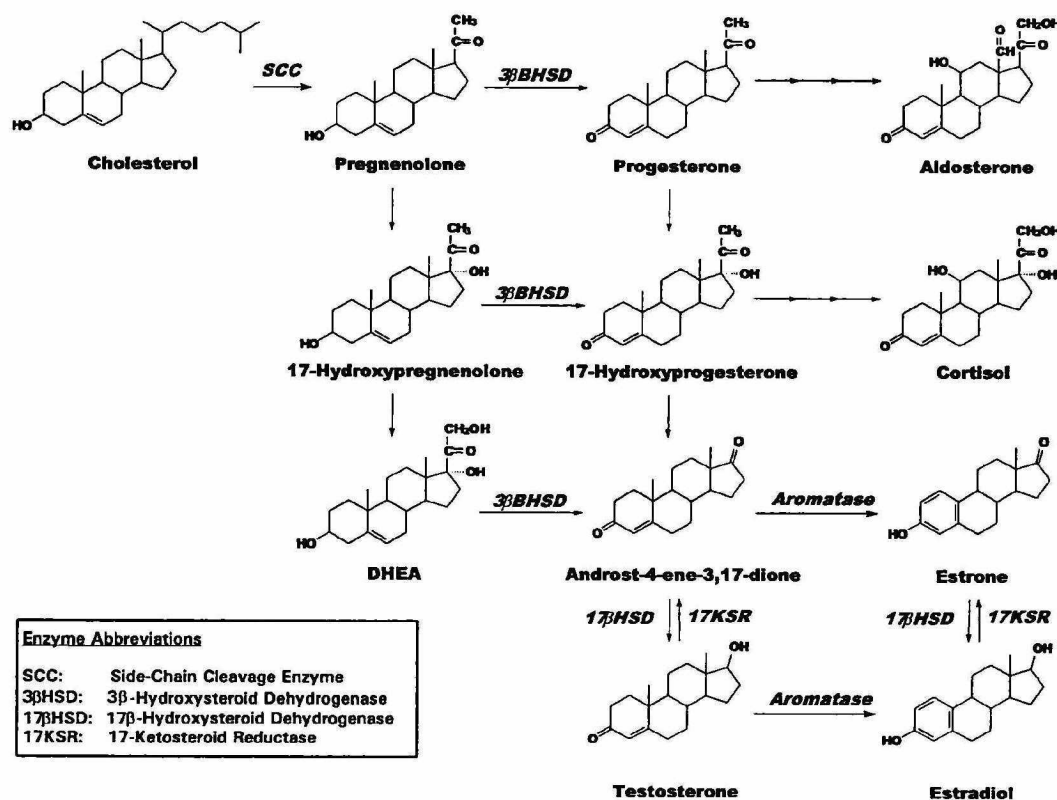
Fig. 1. Steroidogenic pathway.
