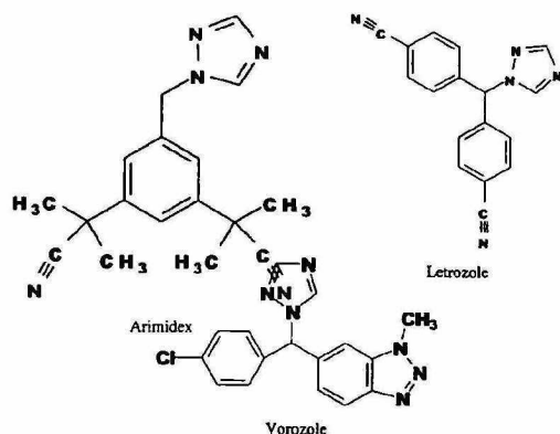
Fig. 3. Triazole nonsteroidal inhibitors.
