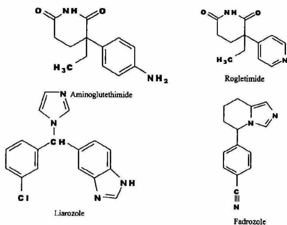
Fig. 2. Piperidinedione and imidazole nonsteroidal inhibitors.
