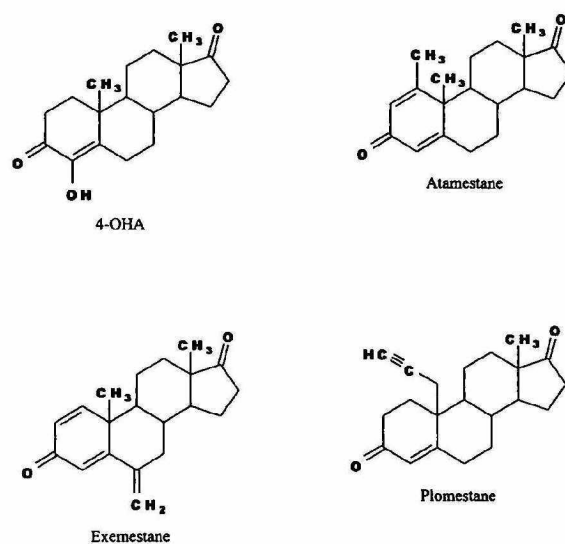
Fig. 4. Steroidal inhibitors.
