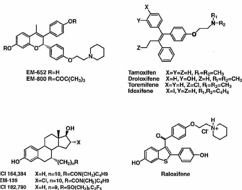
Fig. 1. Antiestrogens—molecular structures.
