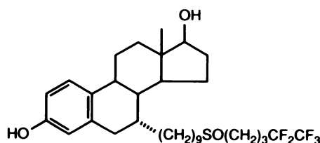
Fig. 1. Structure of pure antiestrogens.
