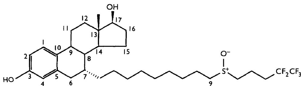
Figure 1. Chemical structure of the estrogen receptor antagonist fulvestrant, 7- \alpha -[9-(4,4,5,5,5 penta fluoropentylsulphinyl) nonyl]estra-1,3,5-(10)-triene-3,17- \beta -diol.
